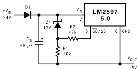
Figure 52. Undervoltage Lockout With Hysteresis for an Inverting Regulator
