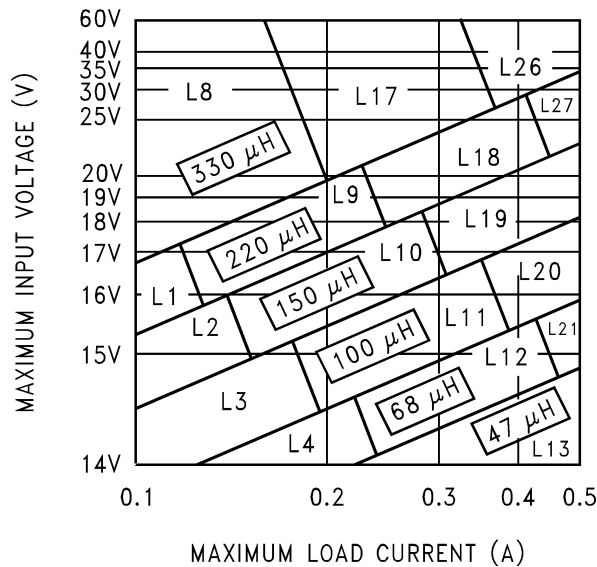
Figure 28. LM2597/LM2597HV-12
