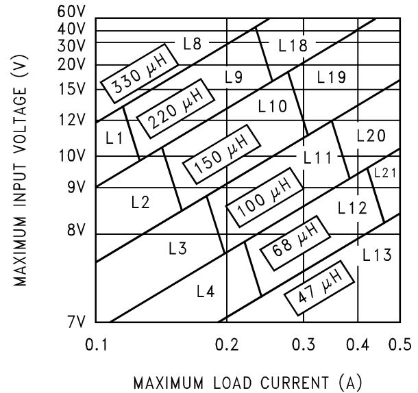
Figure 27. LM2597/LM2597HV-5.0
