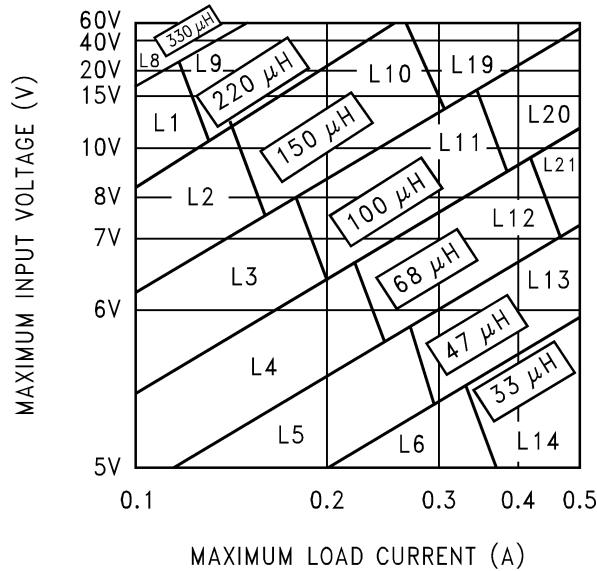
Figure 26. LM2597/LM2597HV-3.3
